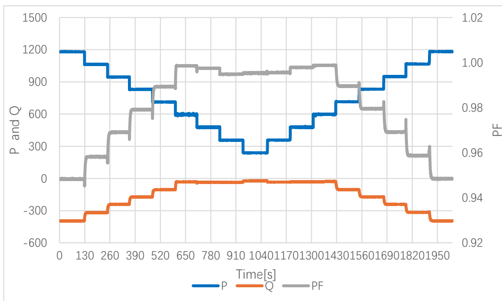
P(t), Q(t), Cosφ(t), Diagram
